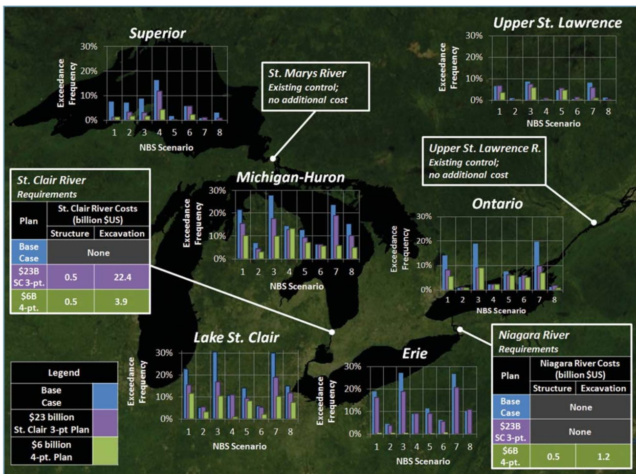
Figure 8-8 Comparison of Performance of the $23 billion St. Clair River Three-point Plan and the $6 billion Four-point Plan Exceedance frequency is equal to the percentage of months simulated for each NBS scenario that exceed the simulated historical extreme water levels. Despite the higher costs (due to greater amounts of excavation required in the St. Clair River), the $23 billion St. Clair River three-point plan performed worse than the $6 billion four-point plan at all six evaluation points and for nearly all NBS scenarios.
