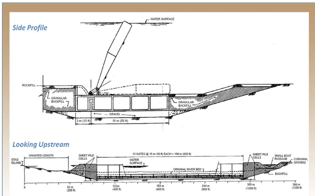
Figure 7-10 Preliminary Design of an Inflatable Flap Gate at Stag Island
