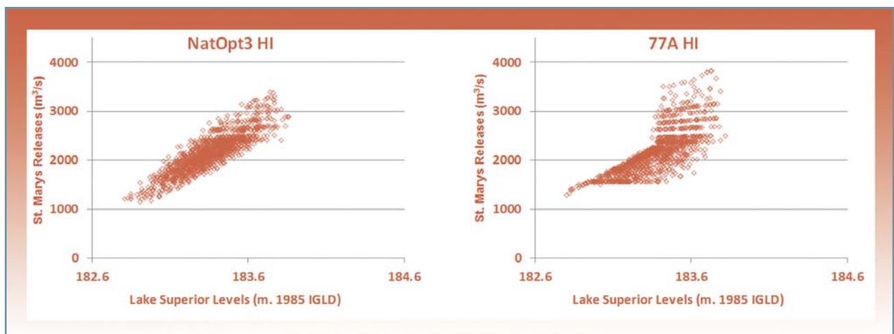
Figure 6-12 Comparison of Natural Flow Levels
